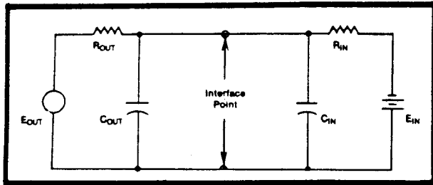
Figure 1—Interchange Circuit.
