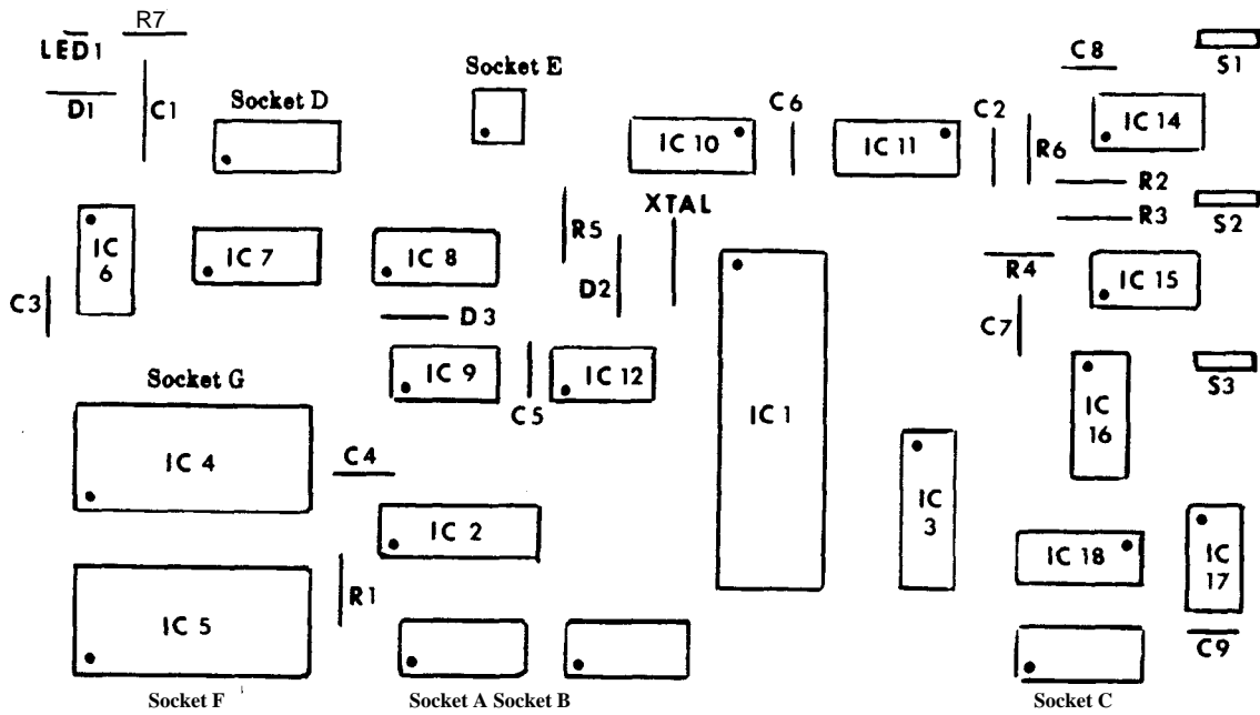
Figure 13: Parts placement.
