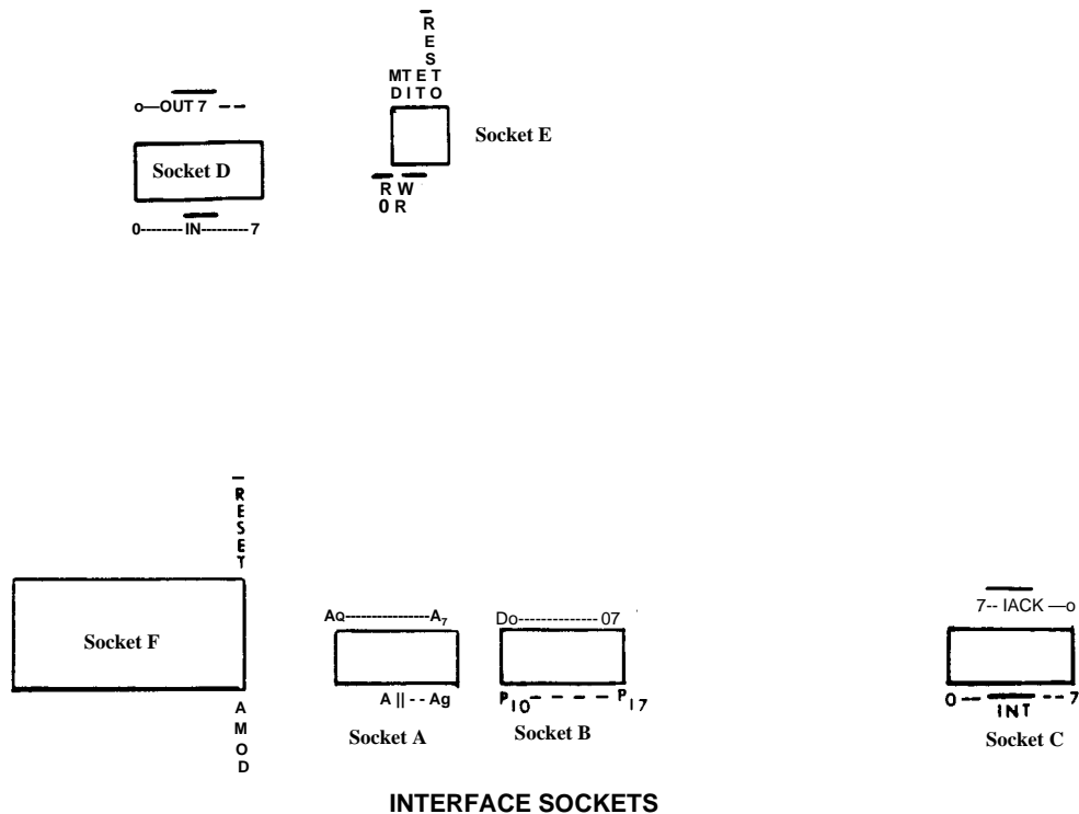
INTERFACE SOCKETS
