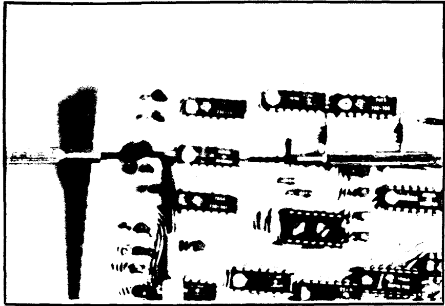
Figure 5: Jeweler's screwdrivers used to pry up an unsoldered DIP. On the left side a resistor acts as fulcrum for the 'lever', on the right another screwdriver at an angle is used with the levered blade threaded between some transistors.
