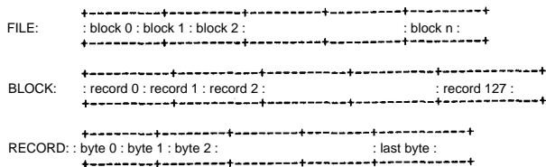
Figure 2. Organization of files by block, record, and byte
