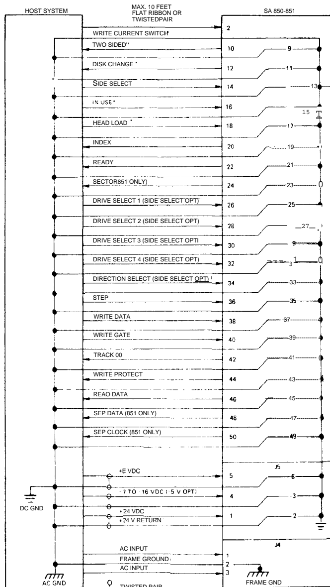
*These lines are alternate input/output lines and they are enabled by plugs. Reference section 7 for uses of these lines. Not shown are pins 4, 6, and 8 which are alternate I/O pins.
