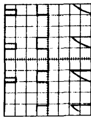
FIGURE 2. Monostable Waveforms
