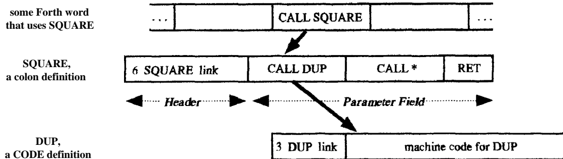
FIGURE 3. SUBROUTINE THREADED CODE
