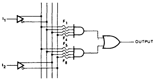
An unprogrammed PAL device has all fuses intact.
