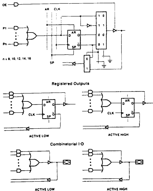
The output logic macrocell makes the PAL22V10 universal, for it can substitute for virtually all of the standard 24-pin PAL devices on the market.
