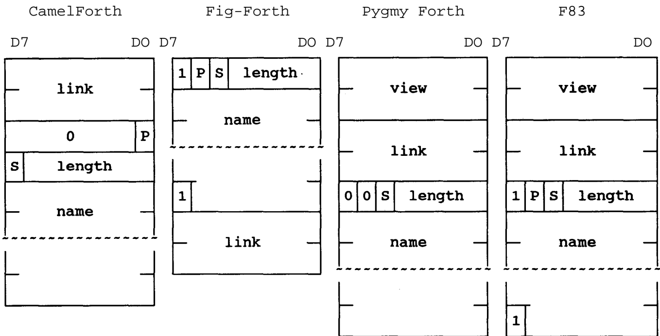
FIGURE 2. HEADER STRUCTURES
