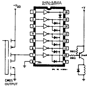
BUFFER FOR HIGH-CURRENT LOAD
