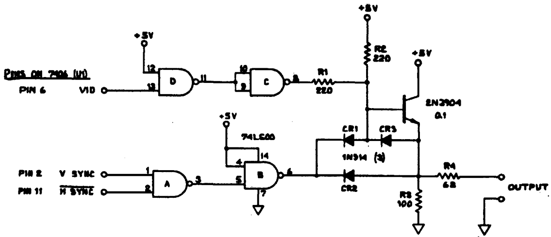
Figure 1. Schematic.
