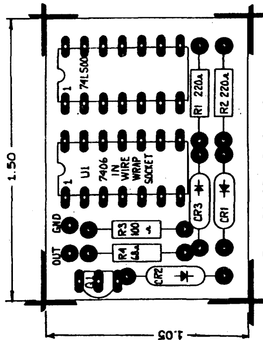
Figure 4. Printed Circuit Board—part layout
