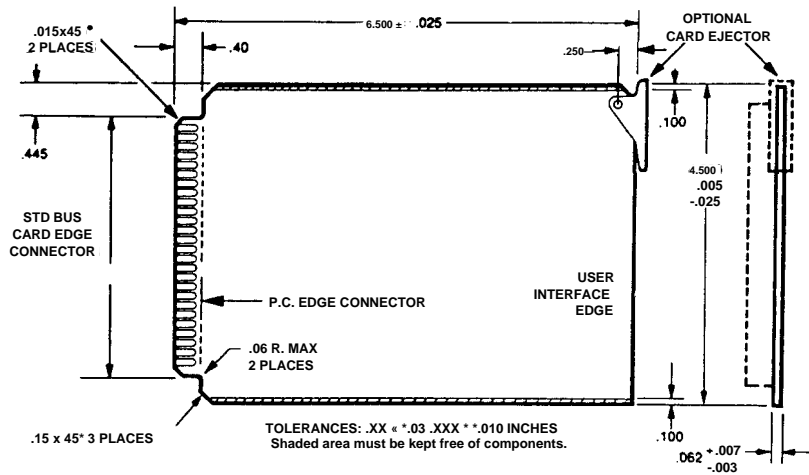
Figure 1-17. Bus Card Outline—inches
