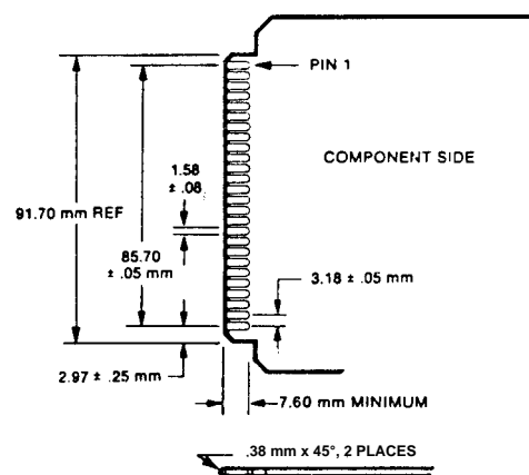
Bus Edge Card Finger Design—Metric
