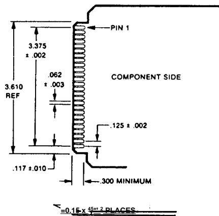
Bus Edge Card Finger Design—inches
