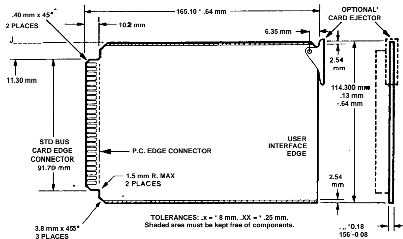
Figure 1-19. Bus Card Outline—Metric
