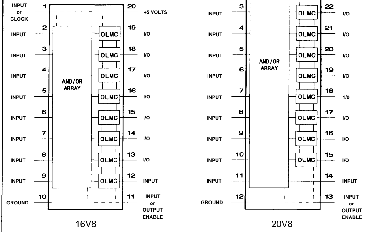
Figure 1. GAL16V8 and GAL 20V8 Architecture
